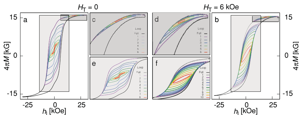
Figure 2. Effects of transverse field on subloop evolution. a,b) Series of nested subloops (colored) inside overall hysteresis loops (black) at H_T = 0 (a) and H_T = 6 kOe (b). c,d) Nested subloops at high longitudinal field (centered on h_l = 18.5 kOe, with loop #1 ranging from 30 to 7 kOe, loop #2 ranging from 29 to 8 kOe, and following that sequence through the final loop which ranges from 20 to 17 kOe). e) Nested low longitudinal field subloops at H_T = 0 , starting at loop #1 with |h_l| = 9 kOe and decreasing for subsequent loops in maximum field by 1 kOe per loop, ending at |h_l| = 3 kOe. f) Nested low longitudinal field subloops at H_T = 6 kOe, starting at loop #1 with |h_l| = 13 kOe and decreasing for subsequent loops in maximum field by 1 kOe per loop, ending at |h_l| = 5 kOe. In the H_T = 0 regime, the high longitudinal field subloops (c) retrace the original outermost subloop (loop #1) unlike the low longitudinal field subloops (e,f), indicating relatively weak disorder. In the H_T = 6 kOe regime, the high longitudinal field subloops (d) deviate from the outermost subloop, indicating strong effective disorder.
