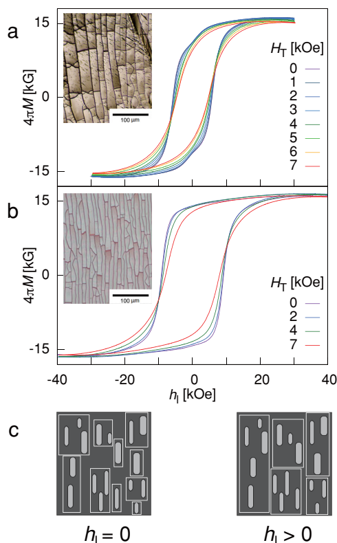
Figure 1. Overview of magnetic behavior of \text{Nd}_2\text{Fe}_{14}\text{B} samples A and B. a,b) Magnetic behavior and structural morphology of two samples of \text{Nd}_2\text{Fe}_{14}\text{B} . Main panels: Magnetic hysteresis loops at T = 300\text{ K} for a series of transverse magnetic fields. Loops are swept out at a constant ramp of 0.75\text{ kOe/min} along the longitudinal (easy) axis while keeping the transverse field fixed. At low (high) longitudinal field, application of a transverse field narrows (broadens) the hysteresis. Insets: Optical micrographs of the \text{Nd}_2\text{Fe}_{14}\text{B} samples' grain structure using dried ferrofluid as a fine-powder contrast-enhancing agent that preferentially settles in the grain boundaries. The magnetic easy axis is in the vertical direction. a) The granular structure is polydisperse in both size and aspect ratio, leading to a clear separation of the high and low field regimes. b) The granular structure consists almost entirely of elongated aspect ratio grains, yielding a squarer hysteresis loop for low transverse fields. In both samples, the grains are tightly packed with little interstitial volume. c) Schematic of magnetic grain coarsening with longitudinal field. As the longitudinal field increases, coarsening effects increase the average size of the magnetic domains, which can span several structural grains and can average out the intergrain disorder.
