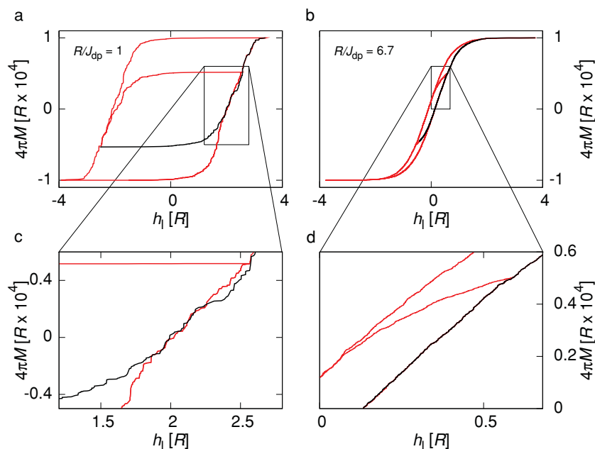
Figure 4. Computer simulations of Return Point Memory for the RFIM with dipolar interactions. a,c) Return point memory in the low random field regime (relative to the strength of the dipolar coupling) with applied field and magnetization in units of the randomness, R . b,d) Return point memory in the high random field regime (relative to the strength of dipolar coupling). Both limits are consistent with the data for \text{Nd}_2\text{Fe}_{14}\text{B} in Figure 3.
